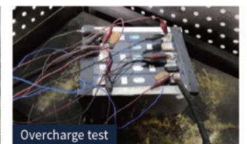
Overcharge test
